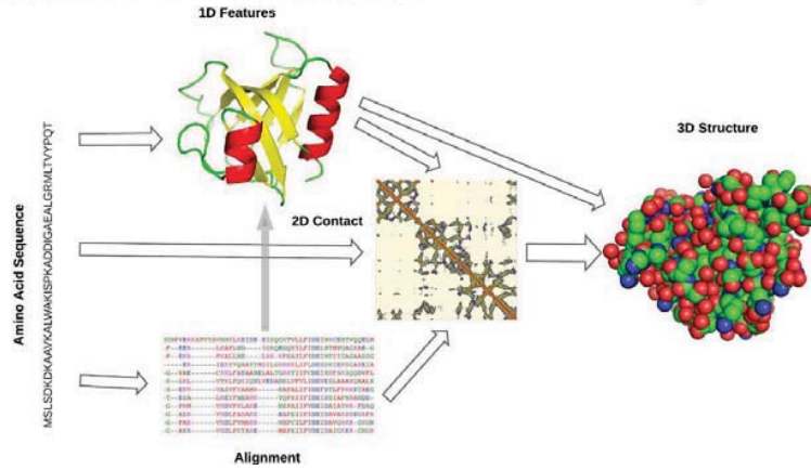
A generic pipeline for ab initio protein structure prediction
