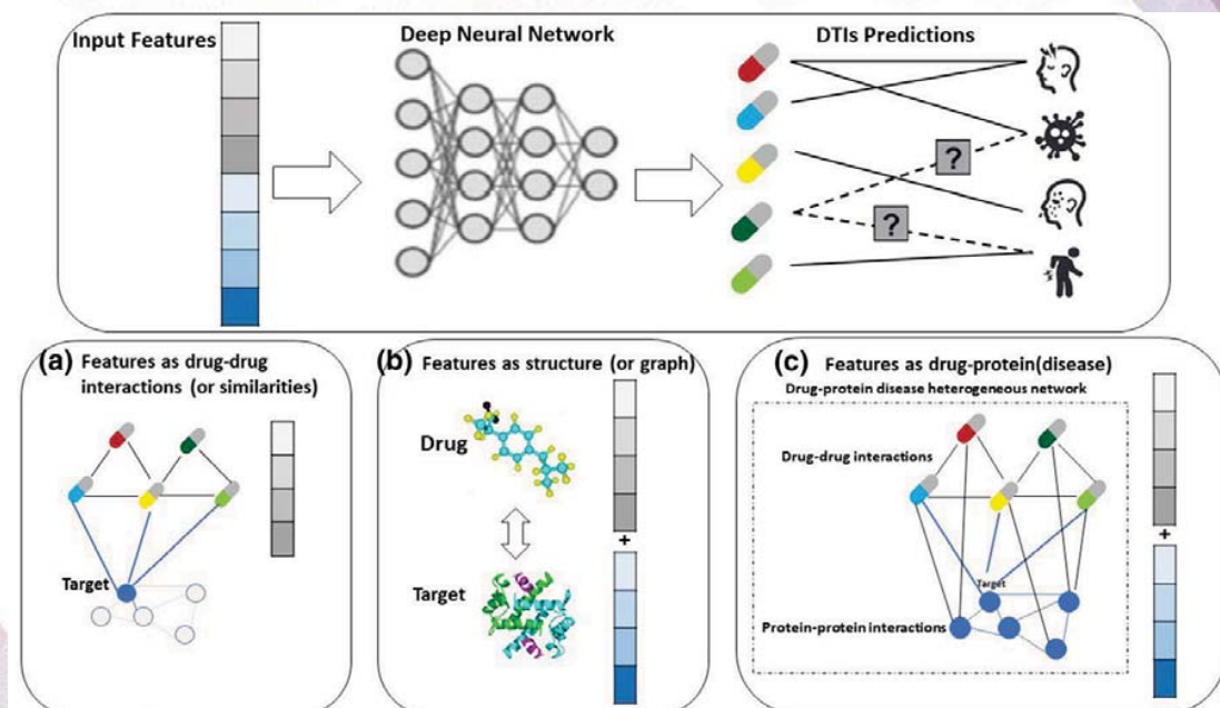
DL models used for predicting the DTIs can be grouped into different categories. (Askr et al, Artificial Intelligence Review 2023)
